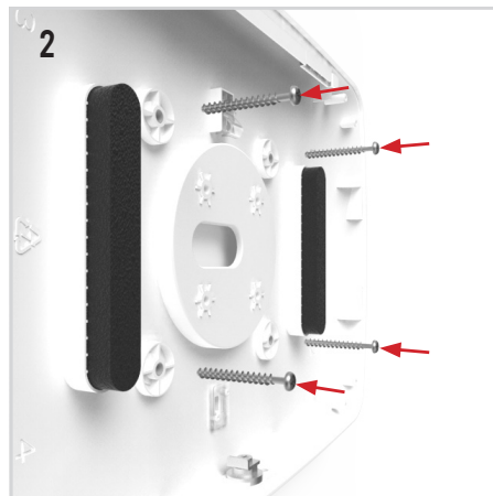
2 Screw the case to the mounting surface using the Vesa holes.
