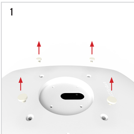
1 Remove the 4 rear rubber pads covering the Vesa mount holes on the case.
